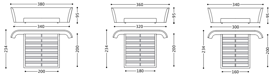
1SMLLA200 1SMLLA180 1SMLLA160
